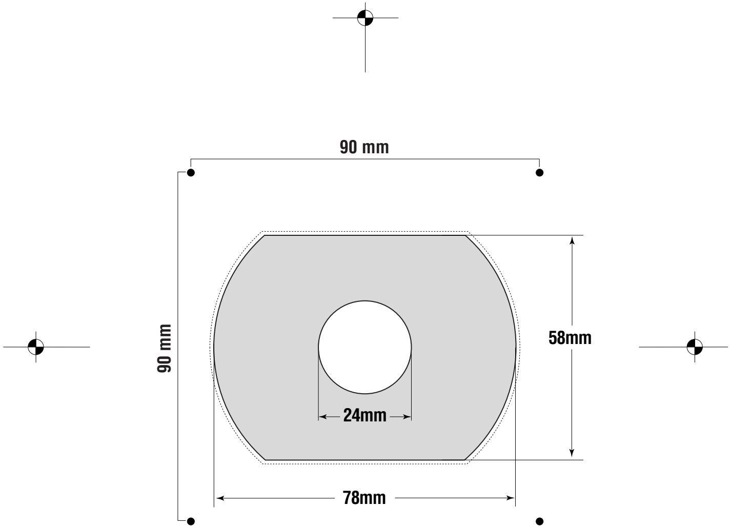
RINK CARD TEMPLATE 80 mm x 60mm (Printable Area: 78mm x 58mm)
